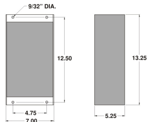
091-187-12-REMOTE Outline Drawing
